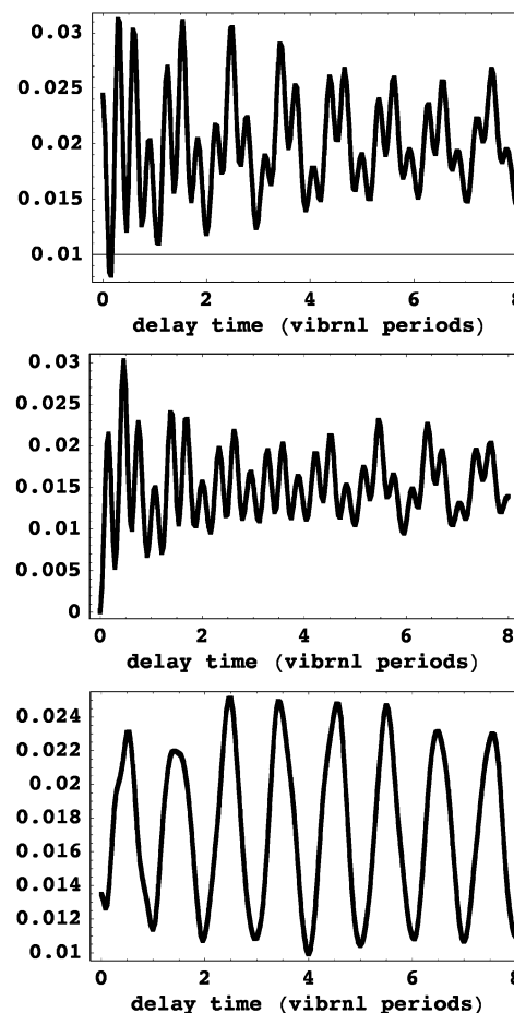
Figure 11. Contributions to polarized emission of Figure 7 with equal site energies and strong coupling. Top: pppp + p'p'p'p' . Middle: pp'p'p + p'ppp' . Bottom: p'p'pp + ppp'p' + p'pp'p + pp'pp' term describing electronic interference between sites. Last quantity is nonnegligible in this strongly coupled system with small vibrational displacements. All vertical axes in identical arbitrary units.
