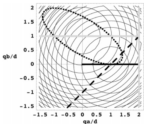
Figure 4. Donor-excited and acceptor-excited electronic potential energy surfaces along with their line of intersection in the case of downhill transfer. Solid line shows the spatial path for wave packet motion after short-pulse excitation to the 1-state, while the elliptical dotted line is the path following a surface-crossing transition to the 1'-state. Lines of emission resonance from donor- and acceptor-excited states at our chosen probe-pulse frequency are shown as vertical and horizontal gray bands, respectively. Note shifted positions of acceptor emission relative to the equal-energy situation of Figure 1.
